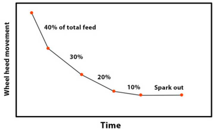
Typical grinding cycle for downfeed and infeed machines
